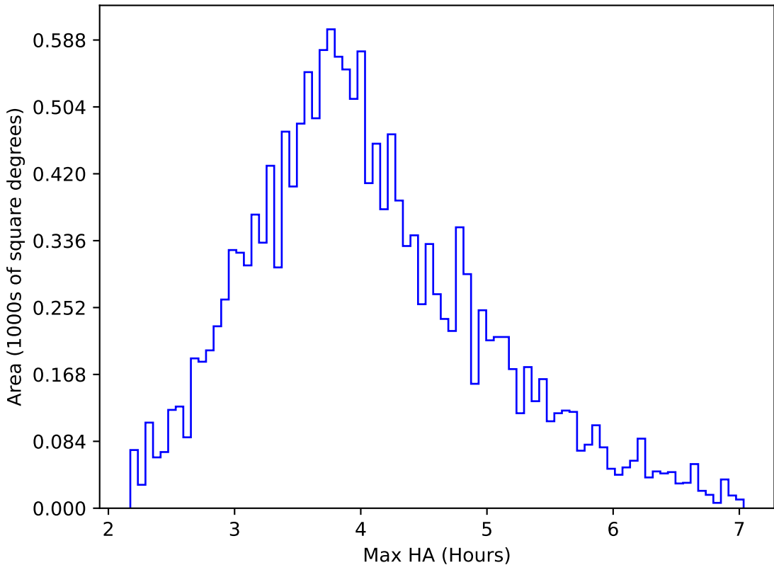
internal_u_expt38_nscale1.2v3.4_10yrs WFD u band: Max HA
