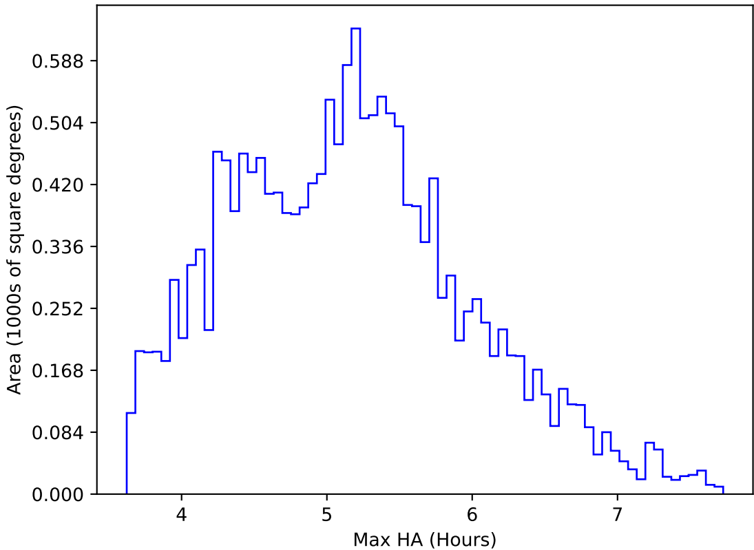
internal_u_expt38_nscale1.2v3.4_10yrs WFD all bands: Max HA
