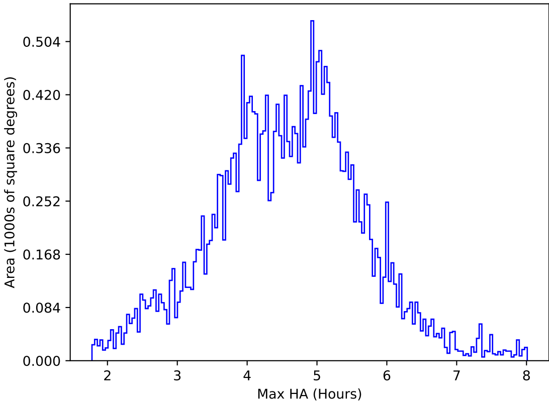
internal_u_expt38_nscale1.2v3.4_10yrs All sky z band: Max HA
