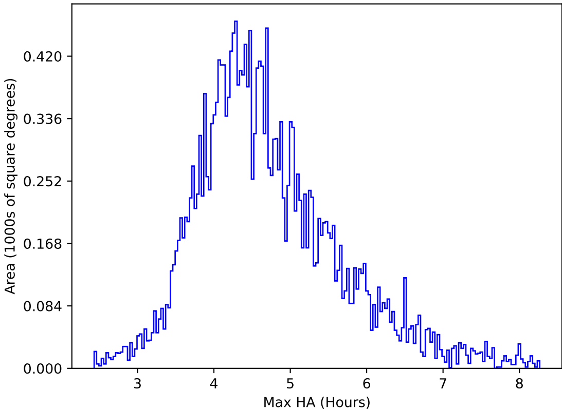
internal_u_expt38_nscale1.2v3.4_10yrs All sky y band: Max HA
