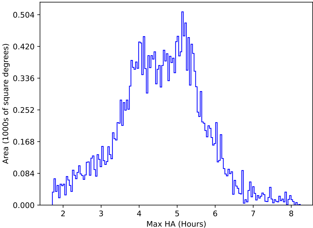
internal_u_expt38_nscale1.2v3.4_10yrs All sky i band: Max HA
