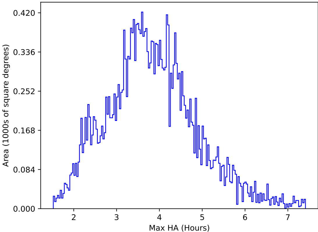
internal_u_expt38_nscale1.2v3.4_10yrs All sky g band: Max HA
