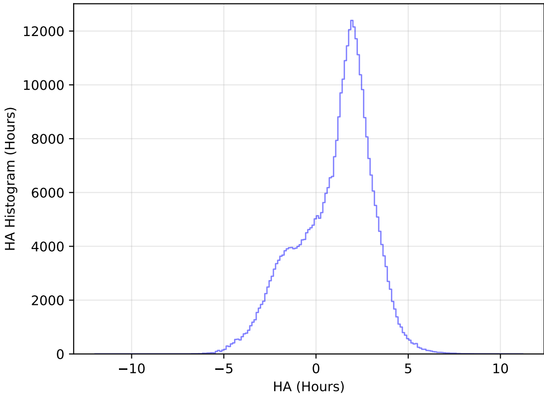
internal_u_expt38_nscale1.2v3.4_10yrs WFD y band: HA Histogram
