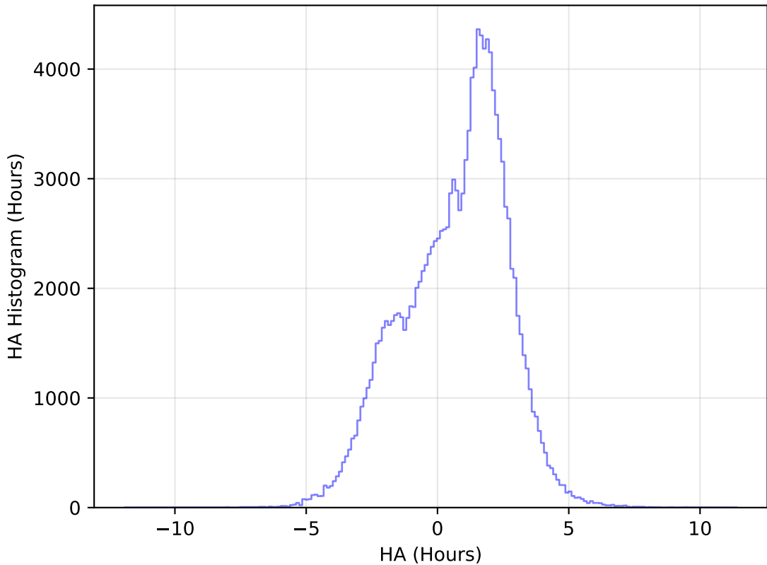
internal_u_expt38_nscale1.2v3.4_10yrs WFD u band: HA Histogram
