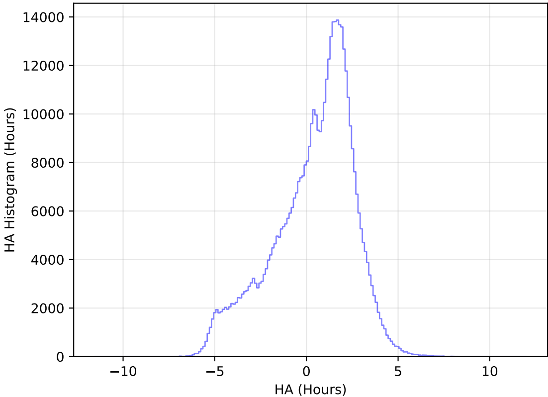
internal_u_expt38_nscale1.2v3.4_10yrs WFD r band: HA Histogram
