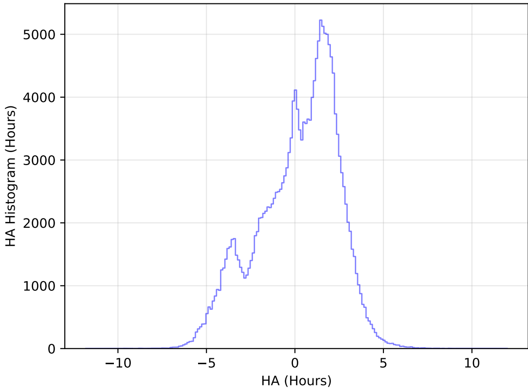
internal_u_expt38_nscale1.2v3.4_10yrs WFD g band: HA Histogram
