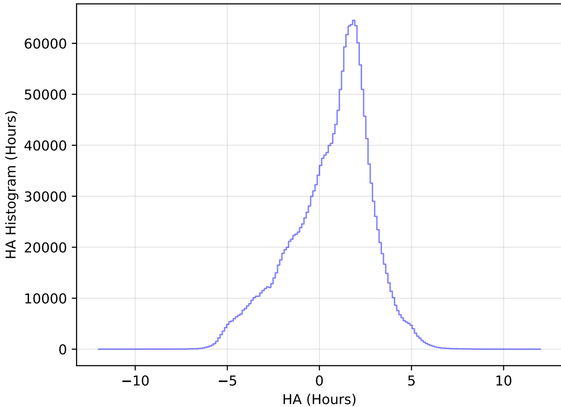
internal_u_expt38_nscale1.2v3.4_10yrs WFD all bands: HA Histogram
