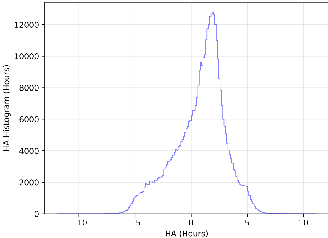
internal_u_expt38_nscale1.2v3.4_10yrs All sky z band: HA Histogram
