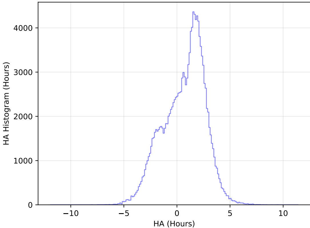
internal_u_expt38_nscale1.2v3.4_10yrs All sky u band: HA Histogram
