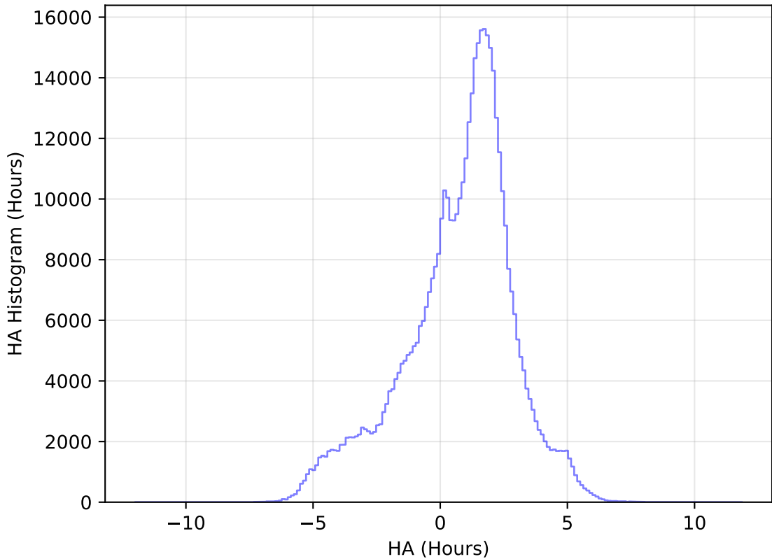
internal_u_expt38_nscale1.2v3.4_10yrs All sky i band: HA Histogram
