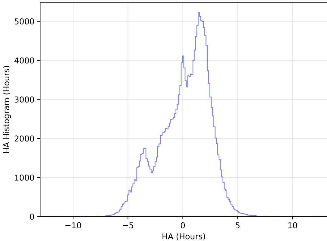
internal_u_expt38_nscale1.2v3.4_10yrs All sky g band: HA Histogram
