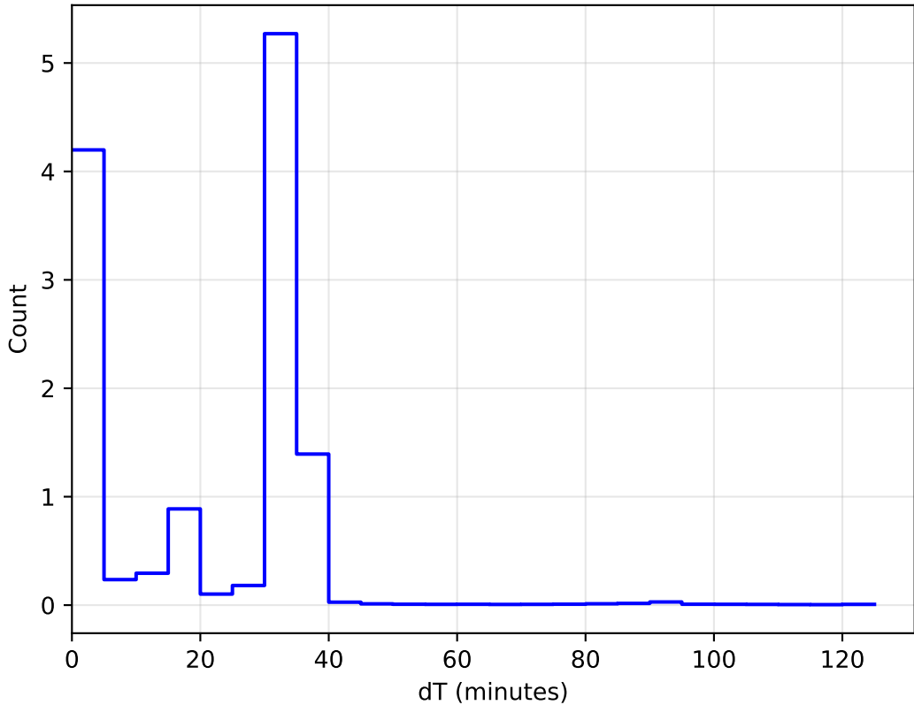
internal_u_expt38_nscale1.2v3.4_10yrs All sky: DeltaT Histogram
