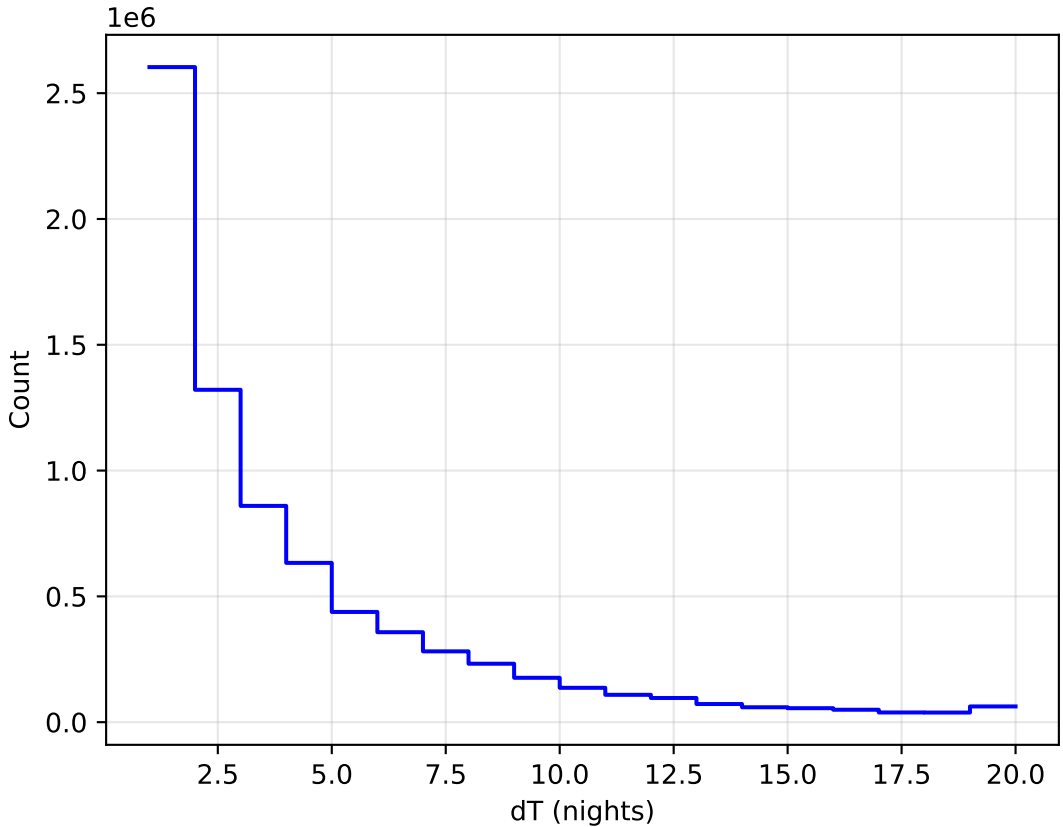
internal_u_expt38_nscale1.2v3.4_10yrs WFD all bands: DeltaNight Histogram
