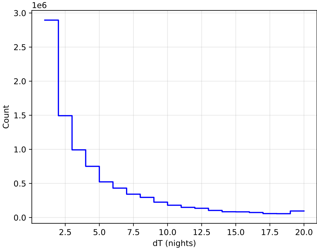
internal_u_expt38_nscale1.2v3.4_10yrs All sky all bands: DeltaNight Histogram
