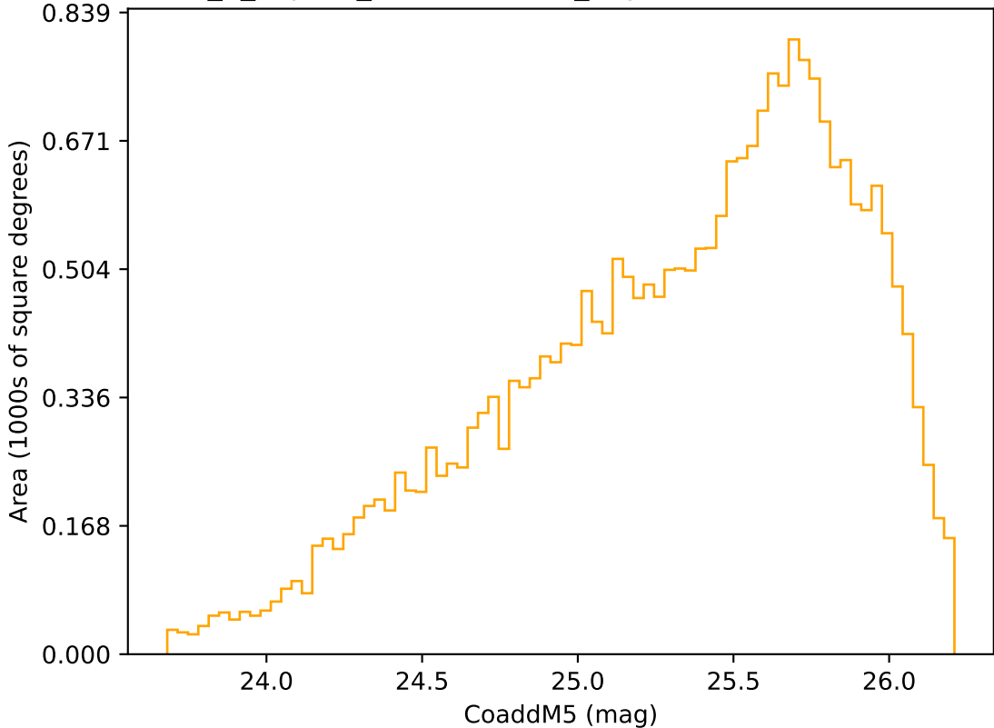
internal_u_expt38_nscale1.2v3.4_10yrs Yr 3-4 r band: CoaddM5
