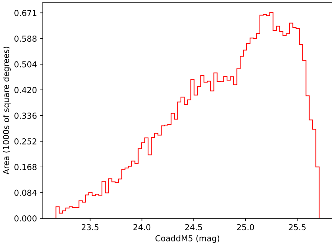
internal_u_expt38_nscale1.2v3.4_10yrs Yr 3-4 i band: CoaddM5
