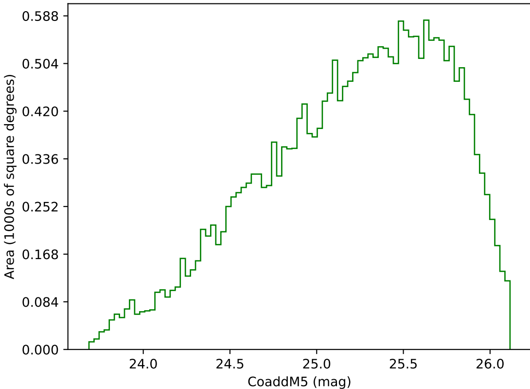
internal_u_expt38_nscale1.2v3.4_10yrs Yr 3-4 g band: CoaddM5
