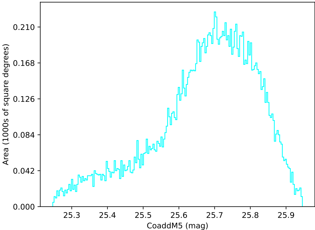
internal_u_expt38_nscale1.2v3.4_10yrs WFD u band: CoaddM5
