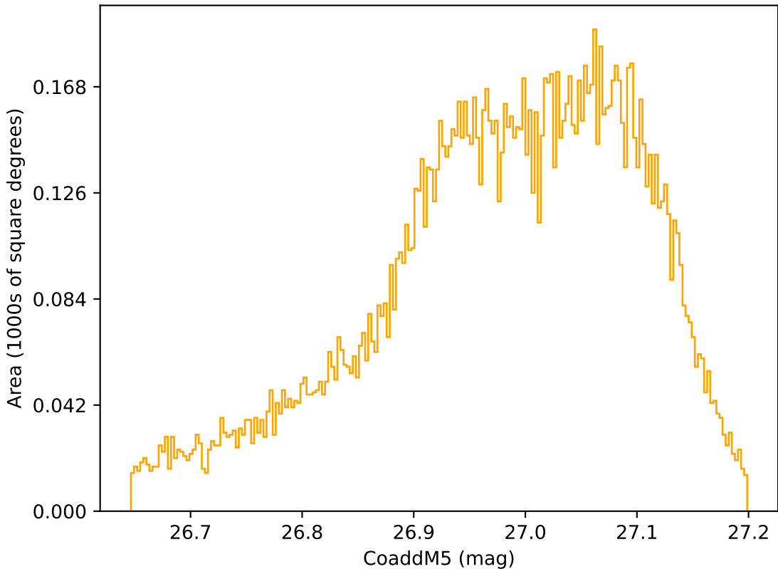
internal_u_expt38_nscale1.2v3.4_10yrs WFD r band: CoaddM5
