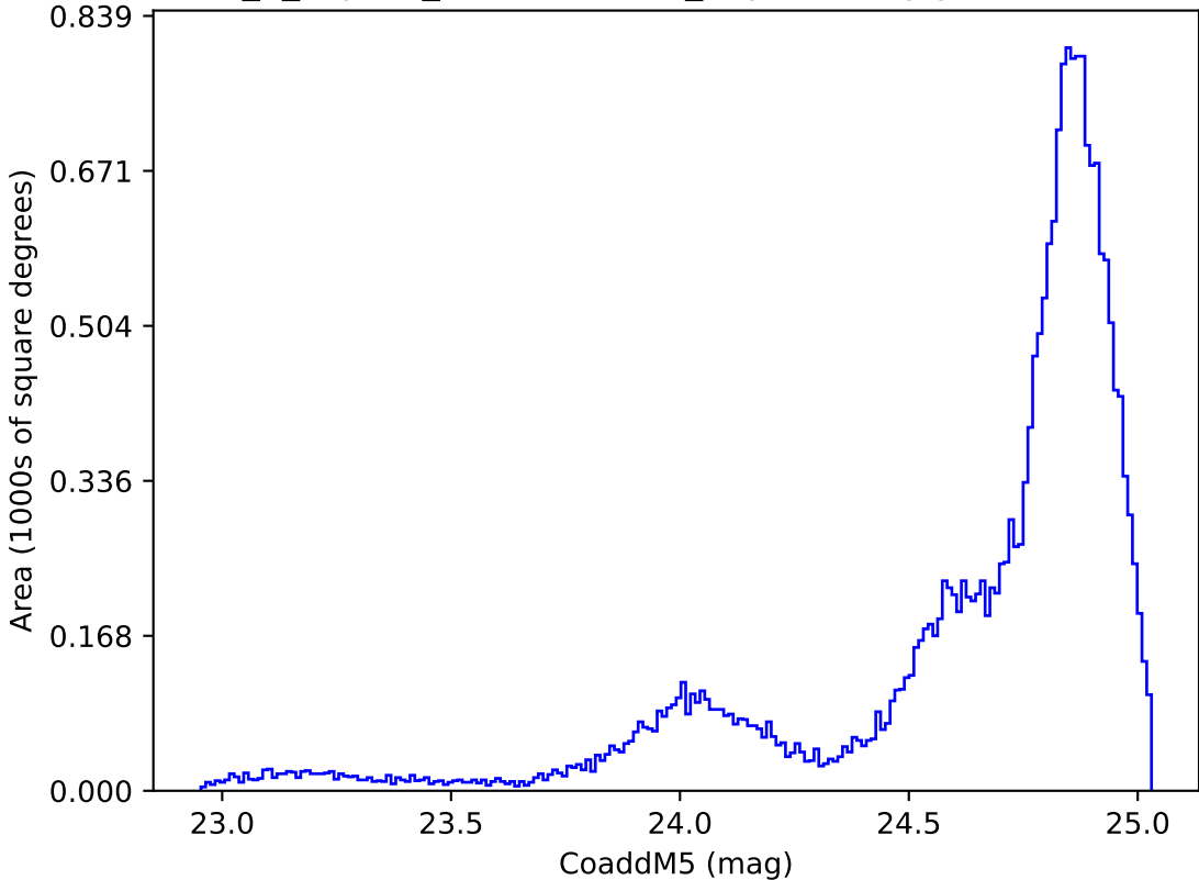
internal_u_expt38_nscale1.2v3.4_10yrs All sky y band: CoaddM5
