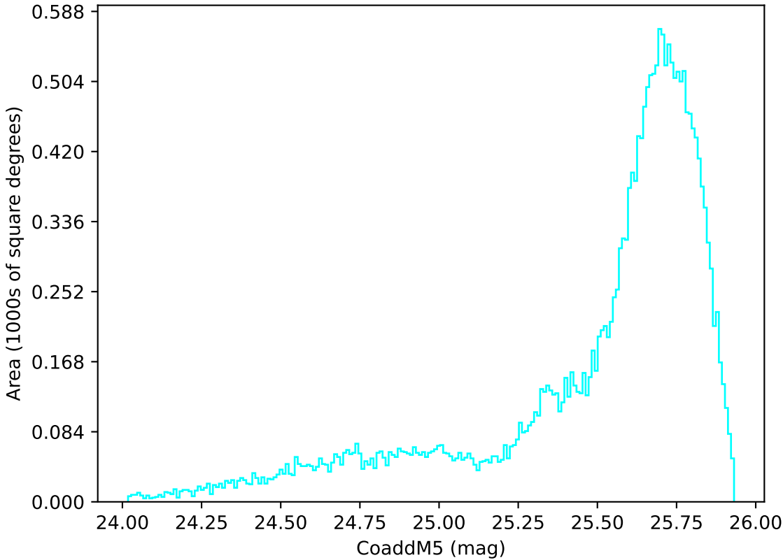
internal_u_expt38_nscale1.2v3.4_10yrs All sky u band: CoaddM5
