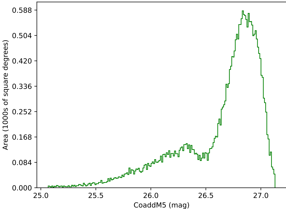
internal_u_expt38_nscale1.2v3.4_10yrs All sky g band: CoaddM5
