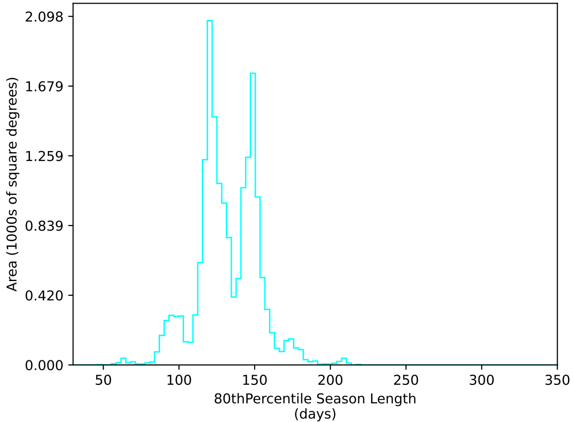
internal_u_expt38_nscale1.2v3.4_10yrs WFD u band: 80thPercentile Season Length
