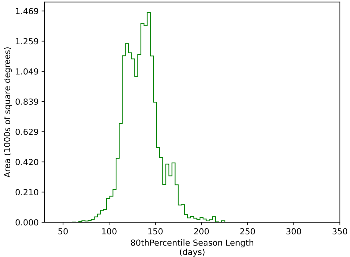
internal_u_expt38_nscale1.2v3.4_10yrs WFD g band: 80thPercentile Season Length
