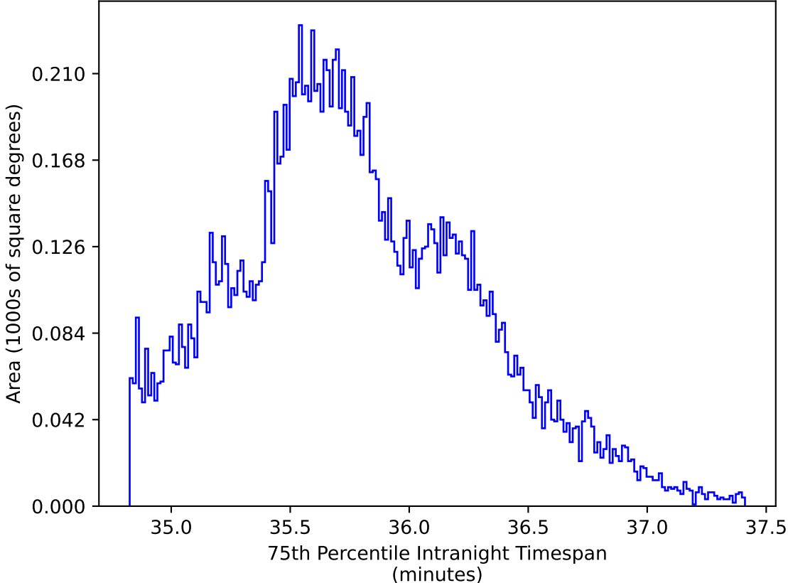
internal_u_expt38_nscale1.2v3.4_10yrs WFD: 75th Percentile Intranight Timespan
