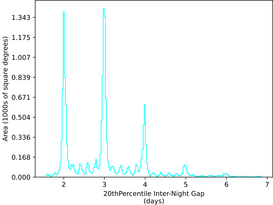
internal_u_expt38_nscale1.2v3.4_10yrs WFD u band: 20thPercentile Inter-Night Gap
