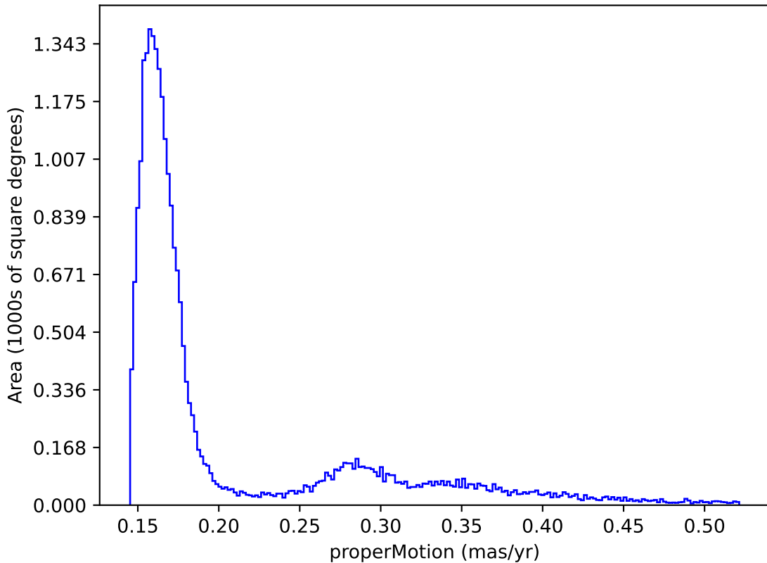
internal_u_expt38_nscale1.2v3.4_10yrs : properMotion
