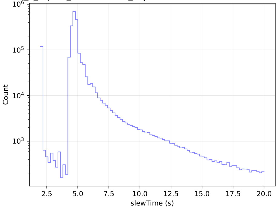
internal_u_expt38_nscale1.2v3.4_10yrs All visits: Zoom Slew Time Histogram
