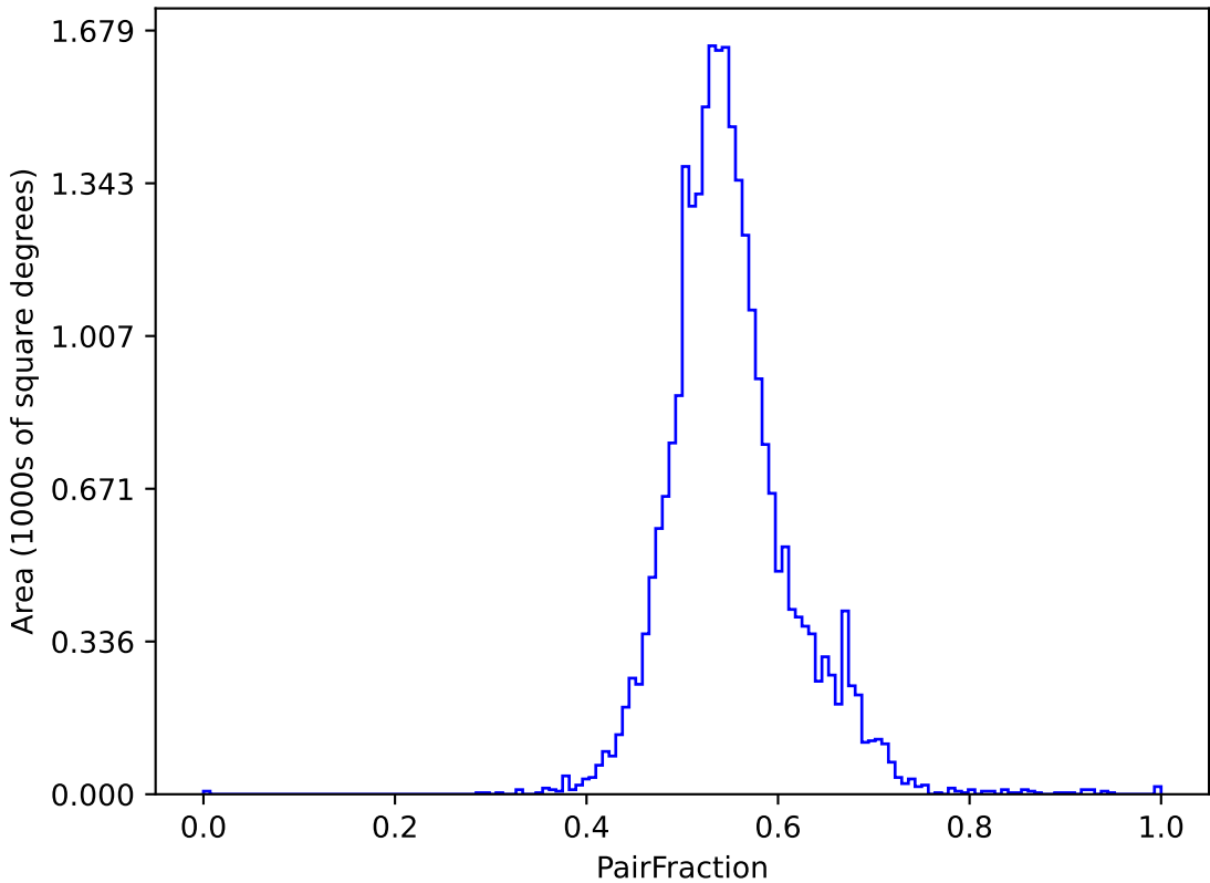
internal_u_expt38_nscale1.2v3.4_10yrs (g or r or i): PairFraction
