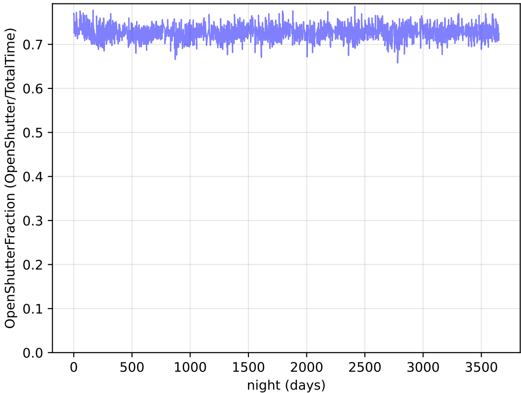
internal_u_expt38_nscale1.2v3.4_10yrs : OpenShutterFraction
