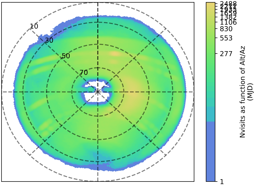
internal_u_expt38_nscale1.2v3.4_10yrs z: Nvisits as function of Alt/Az
