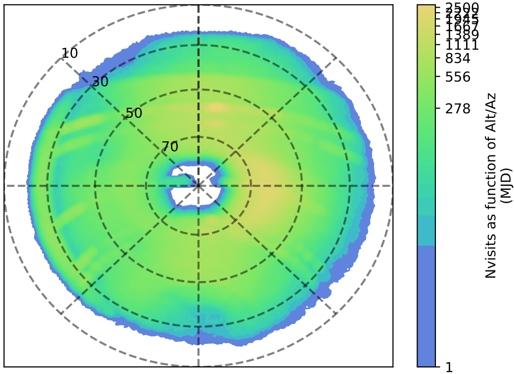
internal_u_expt38_nscale1.2v3.4_10yrs r: Nvisits as function of Alt/Az
