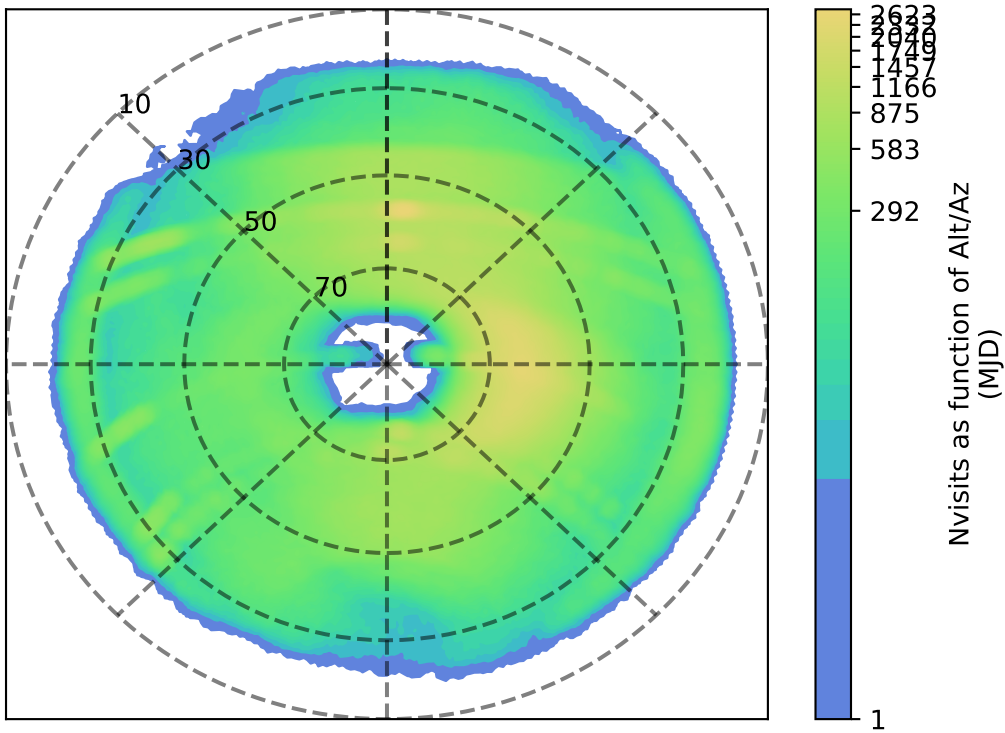
internal_u_expt38_nscale1.2v3.4_10yrs i: Nvisits as function of Alt/Az
