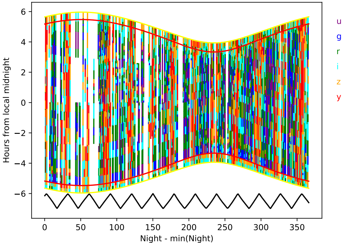
internal_u_expt38_nscale1.2v3.4_10yrs year 9-10: Hourglass
