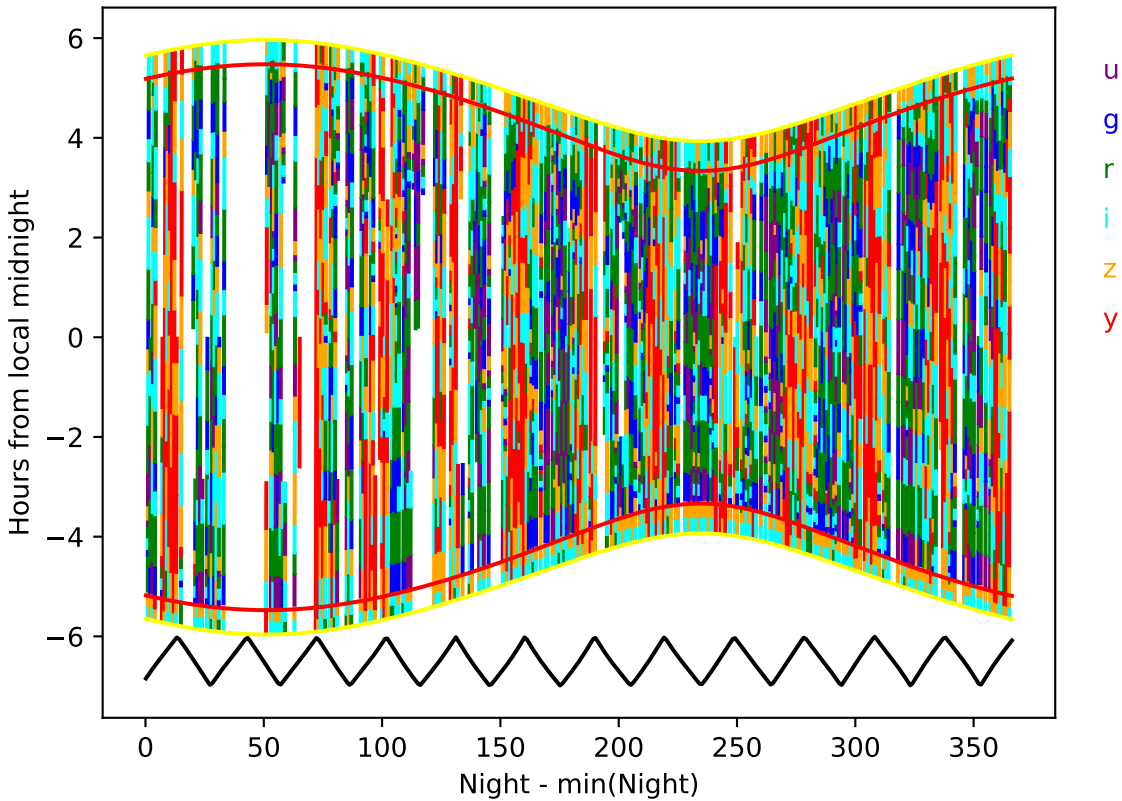
internal_u_expt38_nscale1.2v3.4_10yrs year 8-9: Hourglass
