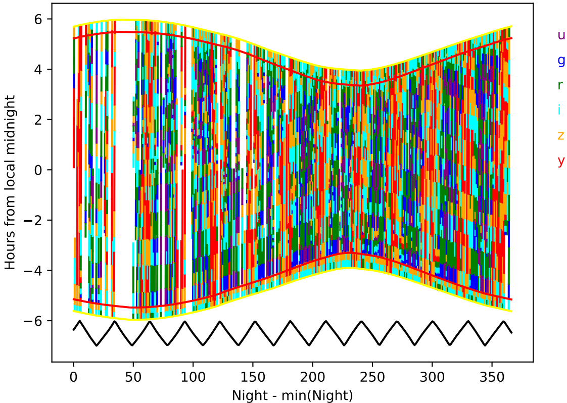
internal_u_expt38_nscale1.2v3.4_10yrs year 6-7: Hourglass
