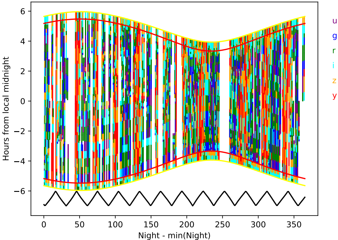
internal_u_expt38_nscale1.2v3.4_10yrs year 5-6: Hourglass
