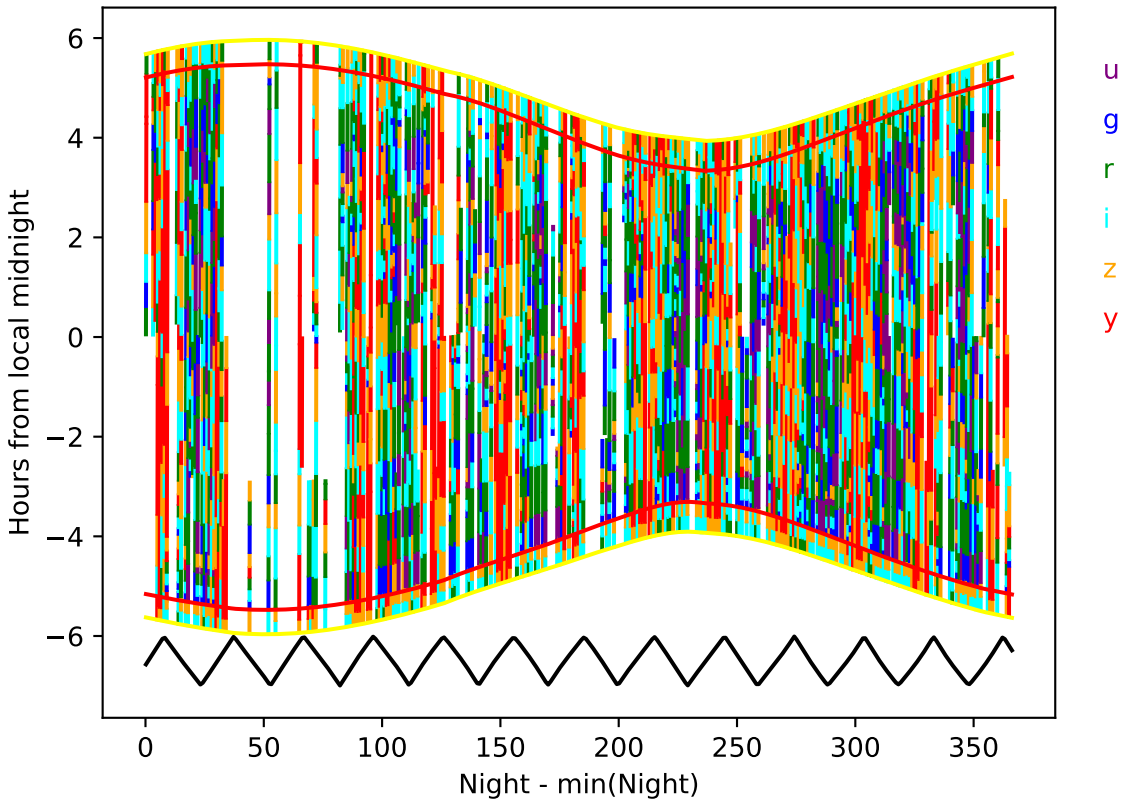
internal_u_expt38_nscale1.2v3.4_10yrs year 3-4: Hourglass
