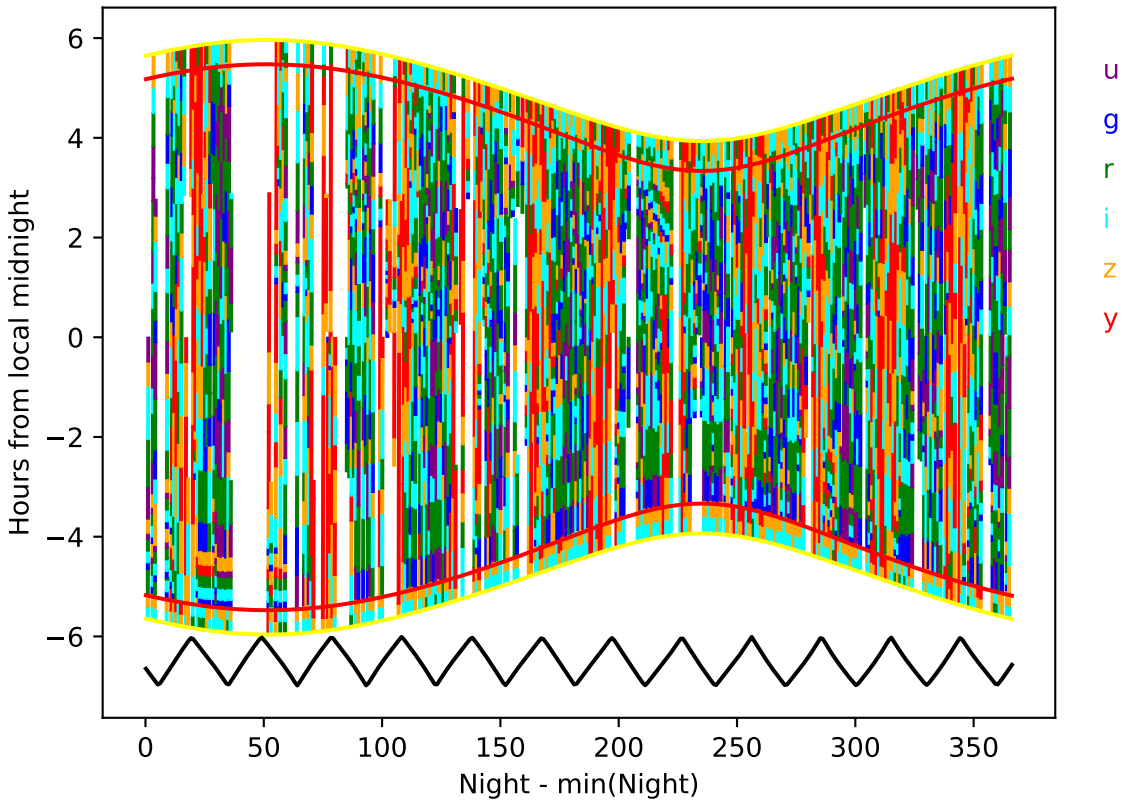
internal_u_expt38_nscale1.2v3.4_10yrs year 2-3: Hourglass
