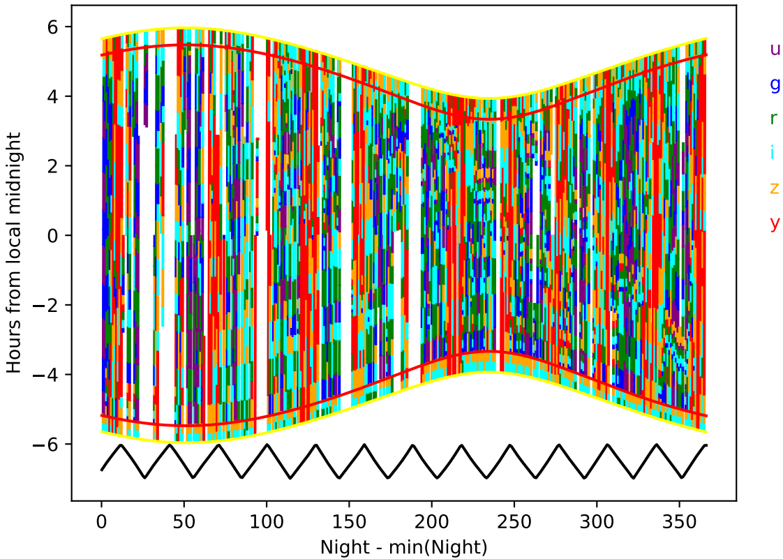
internal_u_expt38_nscale1.2v3.4_10yrs year 0-1: Hourglass
