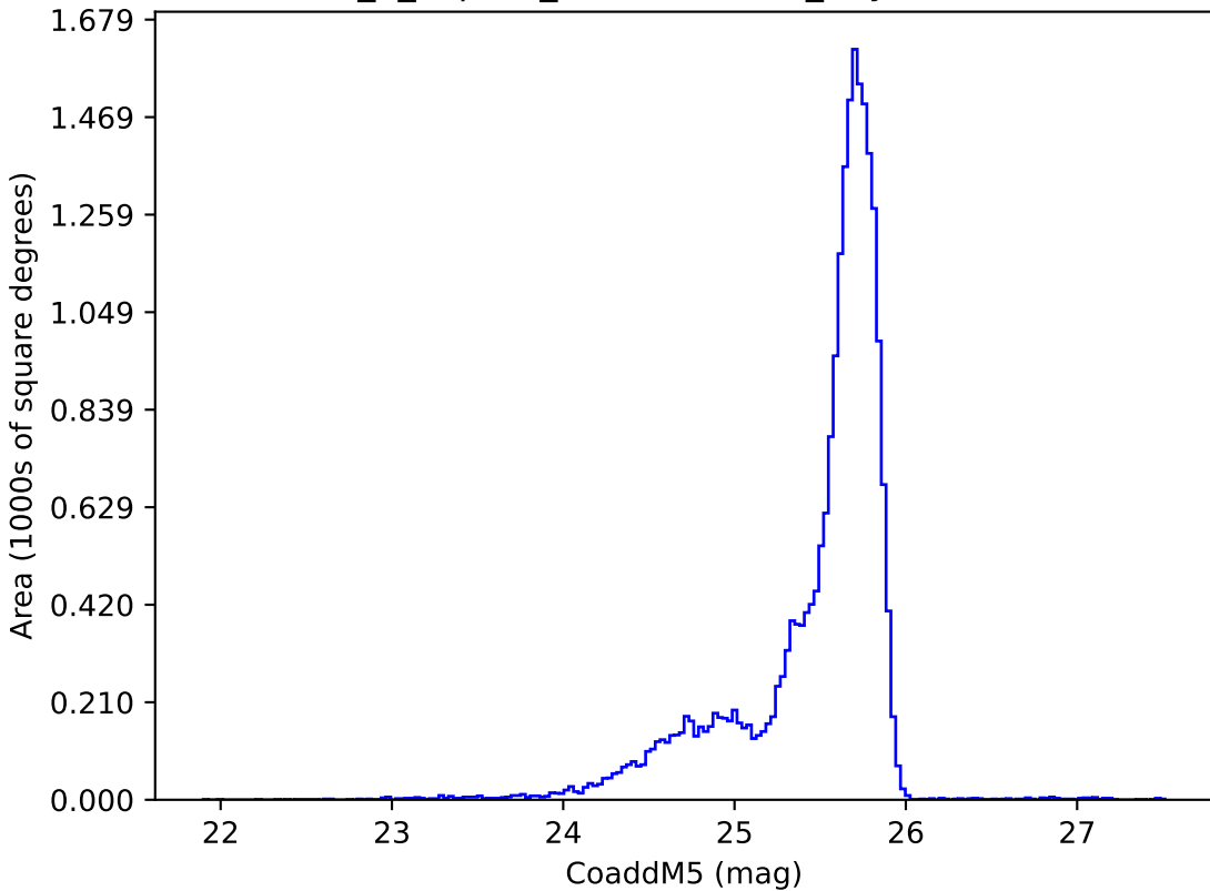
internal_u_expt38_nscale1.2v3.4_10yrs u: CoaddM5
