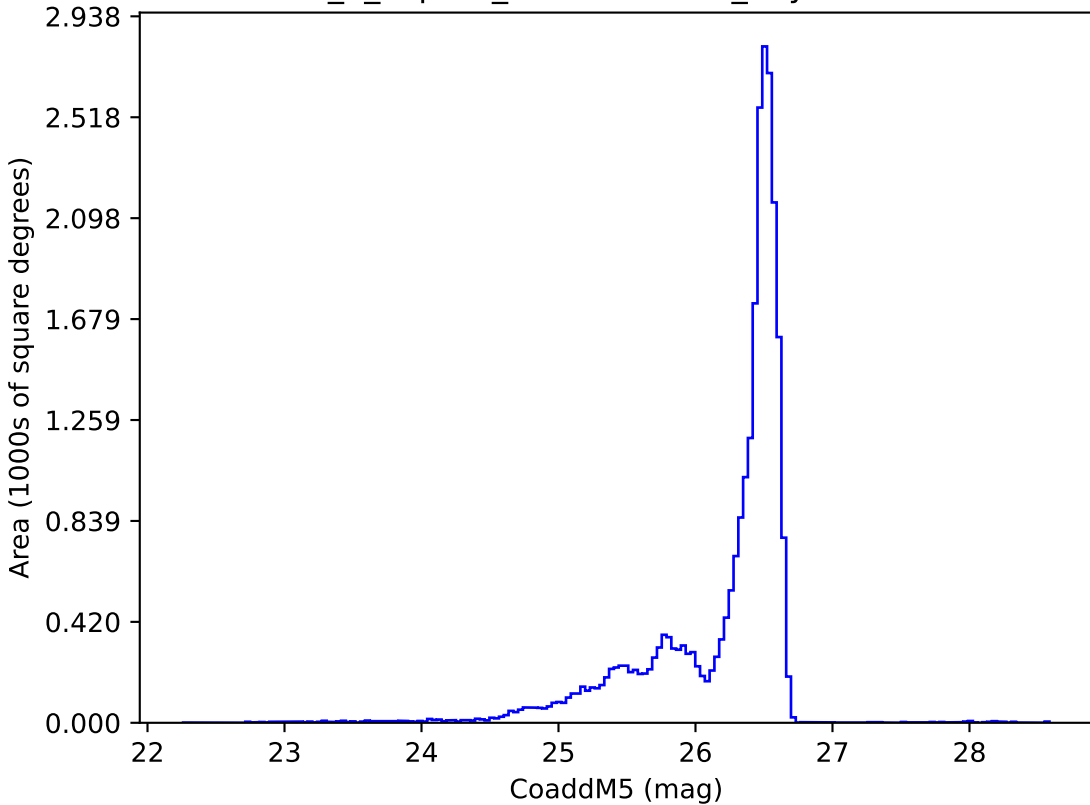
internal_u_expt38_nscale1.2v3.4_10yrs i: CoaddM5
