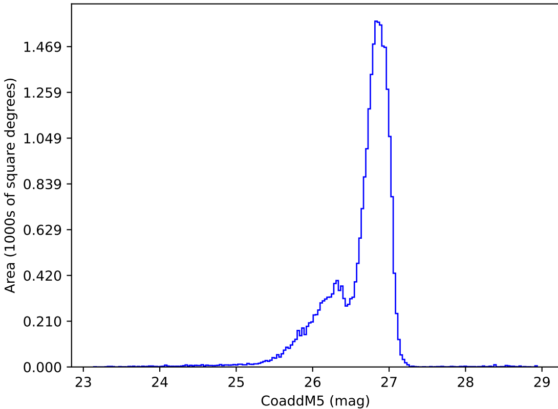
internal_u_expt38_nscale1.2v3.4_10yrs g: CoaddM5
