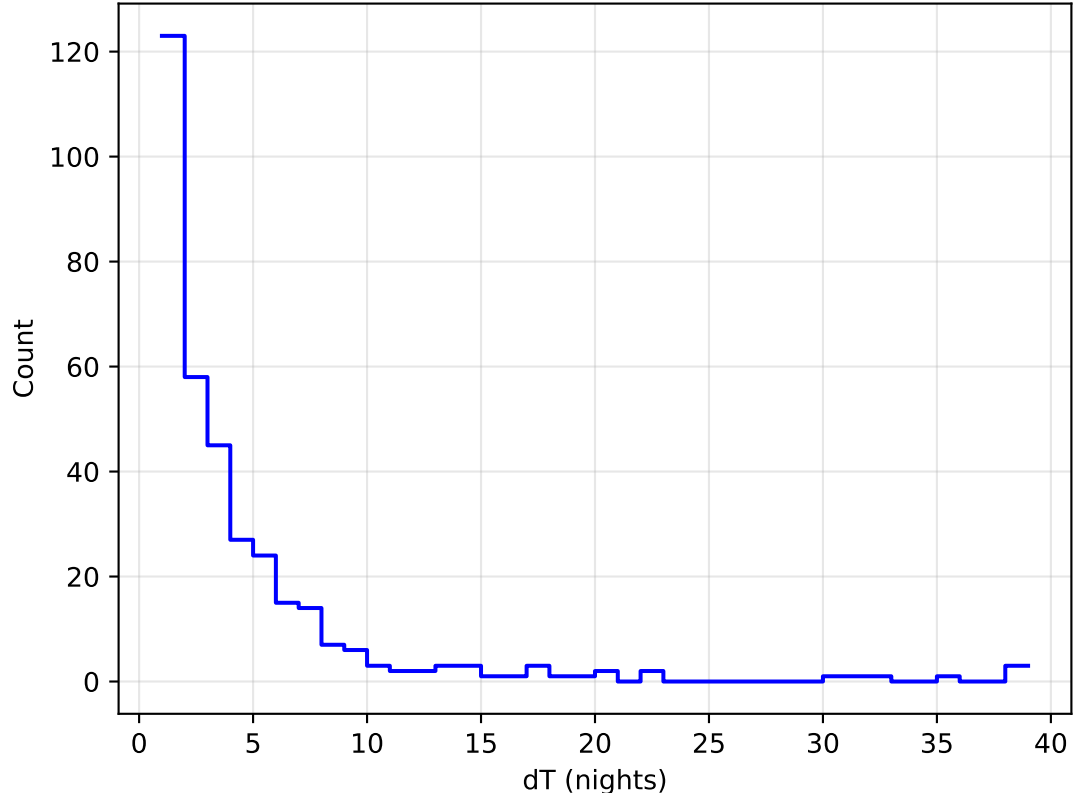
internal_u_expt38_nscale1.2v3.4_10yrs all bands: DD:WFD Delta Nights Histogram
