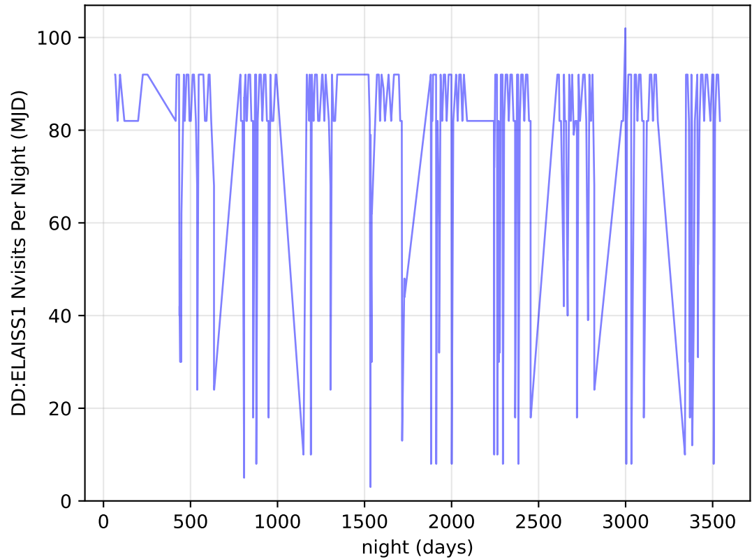
internal_u_expt38_nscale1.2v3.4_10yrs all bands: DD:ELAISS1 Nvisits Per Night
