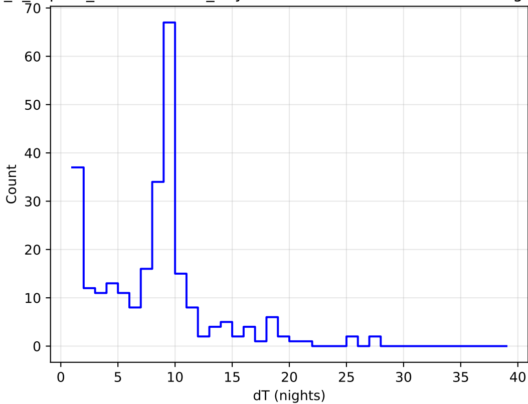
internal_u_expt38_nscale1.2v3.4_10yrs all bands: DD:ELAISS1 Delta Nights Histogram
